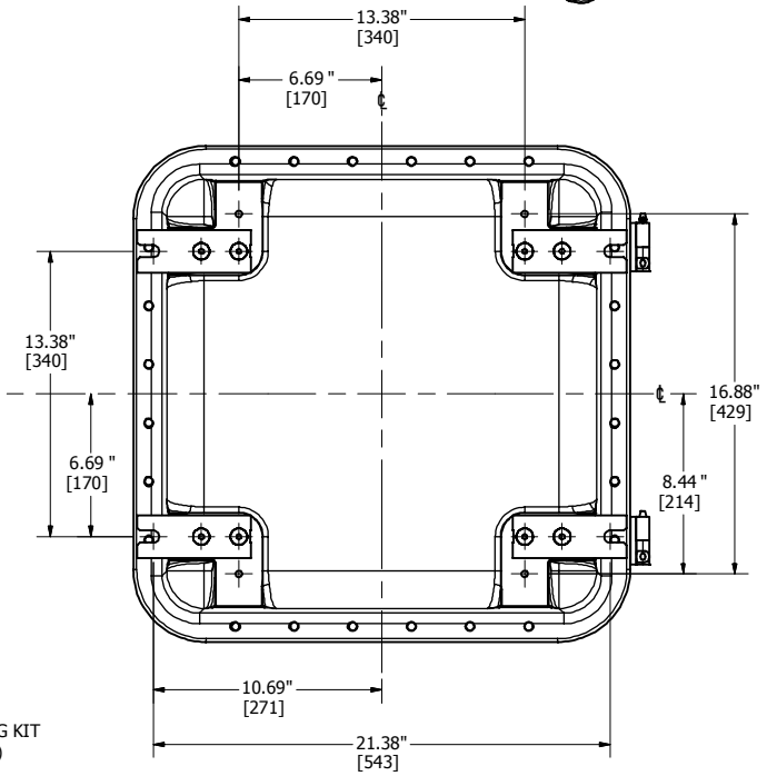
MOUNTING FEET
